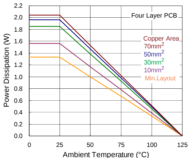
Figure 7. Derating Curves for RT8292A Package
