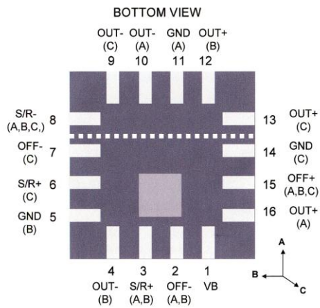
HMC1053 Pinout
