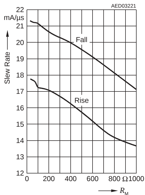
Slew Rate without C = f(R_M)
