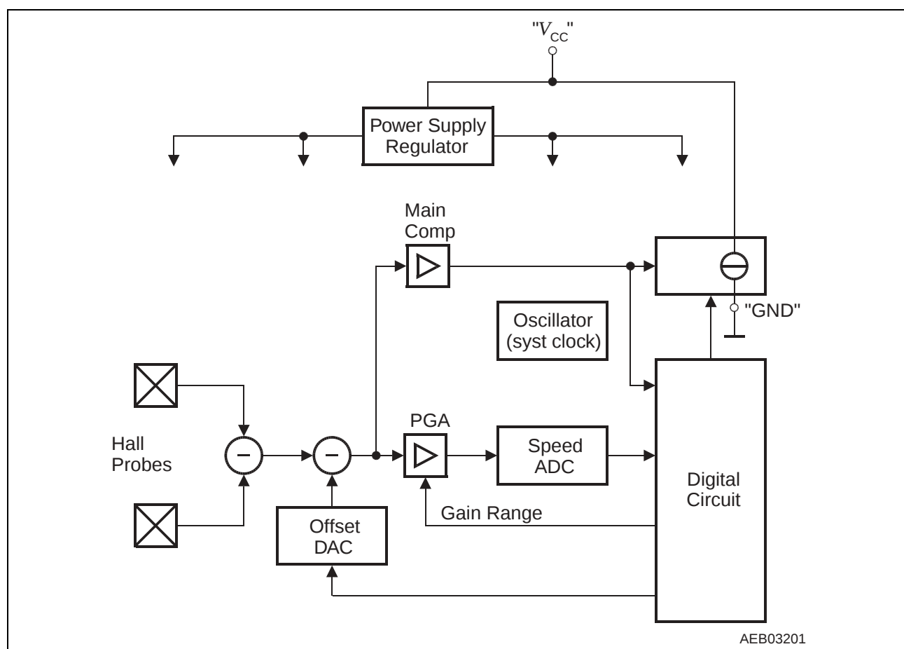
Figure 2 Block Diagram
