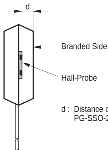
Figure 6 Distance Chip to Upper Side of IC
