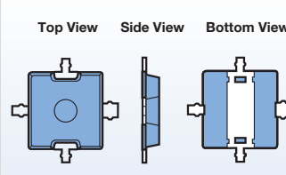
79A Package (4.2 x 4.4 x 0.9)
