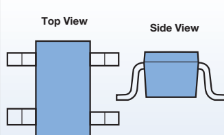
39 Package (1.5 x 2.9 x 1.1)
