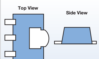
M02 Package (2.45 x 4.5 x 1.5)
