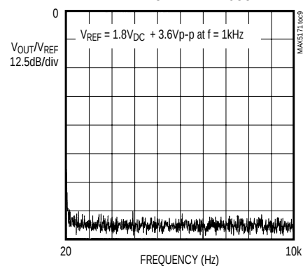
REFERENCE FEEDTHROUGH
