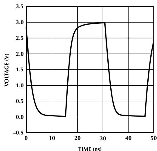
Figure 2: Typical 32 MHz Square wave output signal (1k \Omega +10pF load, VCC = 3.3V)
