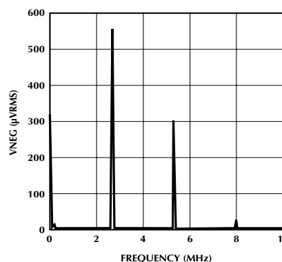
Figure 6: Negative voltage output ripple ( \mu V) (using 100nF bypass and reservoir capacitance)
