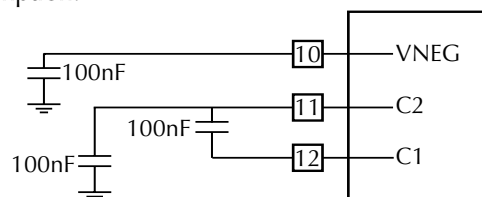
Figure 4: Typical C1 and C2 Noise Shunt Configuration
