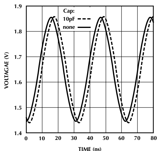
Figure 3: Typical 32 MHz sine wave output signal (1k \Omega +0pF load, and 1k \Omega +10pF load, VCC = 3.3V)
