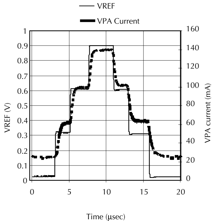
Figure 12: VPA output vs VREF (TRANSMIT mode, R_{EXT} = 12k\Omega , capacitance on VBIAS = 3.3nF)
