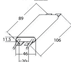
3G3AX-REM00K1□□□
