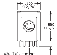
Actuator Shown In Pos. 1 Terminals & Support
