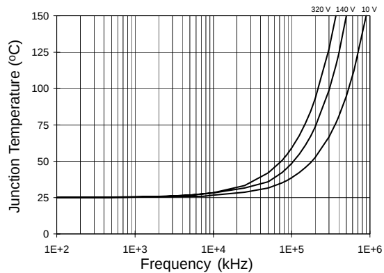
Figure 35. IRS2110S/IRS2113S T_J vs. Frequency (IRFPE50) R_{\text{GATE}} = 10 \Omega , V_{\text{CC}} = 15 \text{ V}
