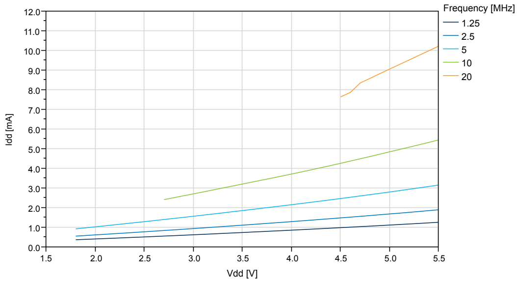
Figure 32-4. ATtiny406: Active Supply Current vs. V_{DD} (f=[1.25, 20] MHz OSC20M) at T=25 ^{\circ}\text{C}
