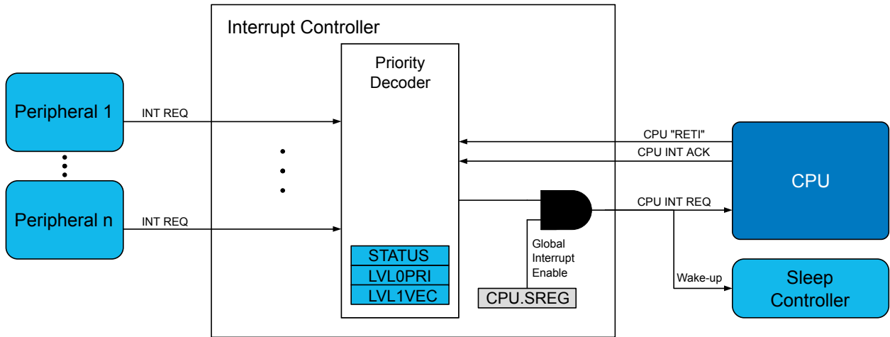
Figure 13-1. CPIINT Block Diagram
