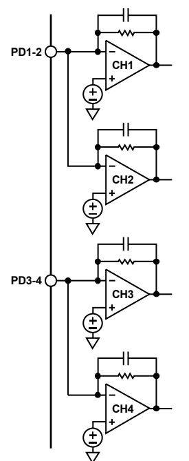
INPUT CONFIGURATION FOR REGISTER 0x14[11:8] = 5 REGISTER 0x14[7:4] = 5
