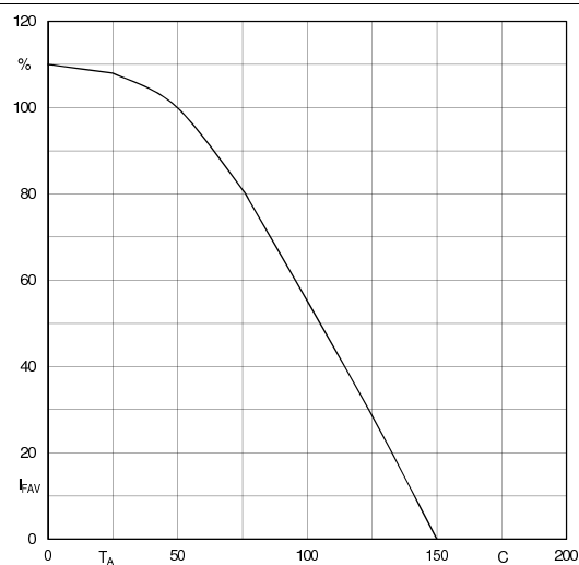
Fig.2: Rated forward current vs. ambient temperature 4)
