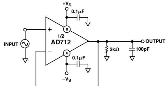
TPC 20. THD Test Circuit
