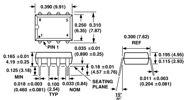
CERDIP (Q-8)
