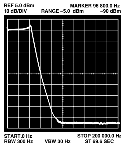
Figure 19. High Frequency Response for 9-Pole Chebychev Filter
