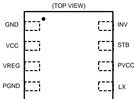
Figure 2. Pin Configuration
