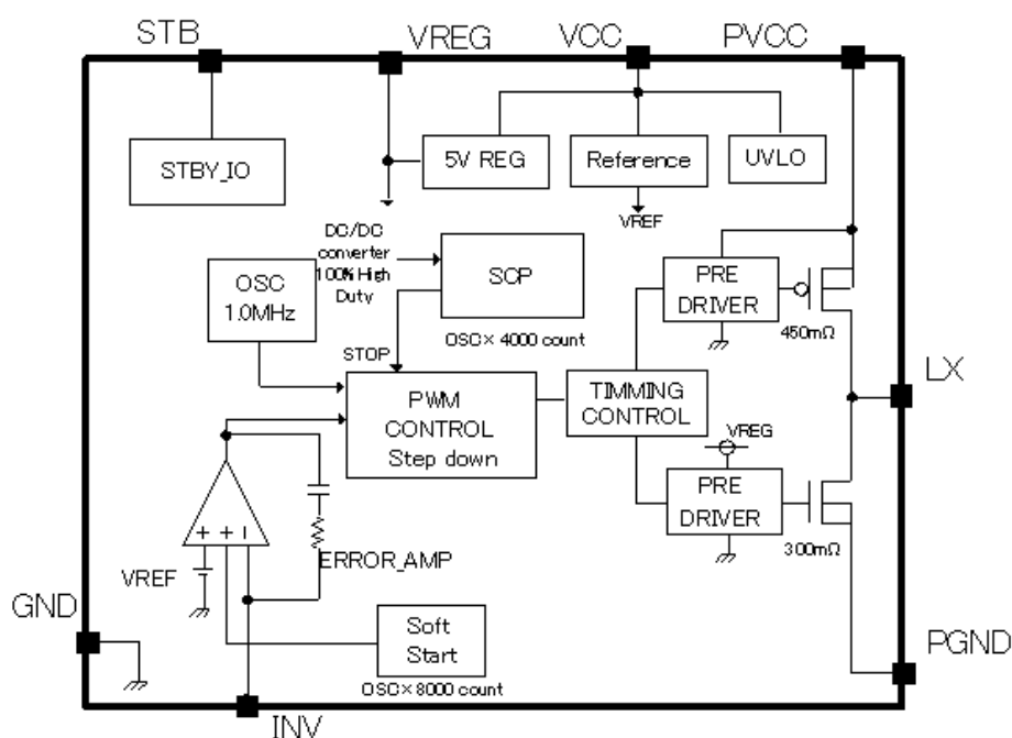
Figure 3. Block Diagram
