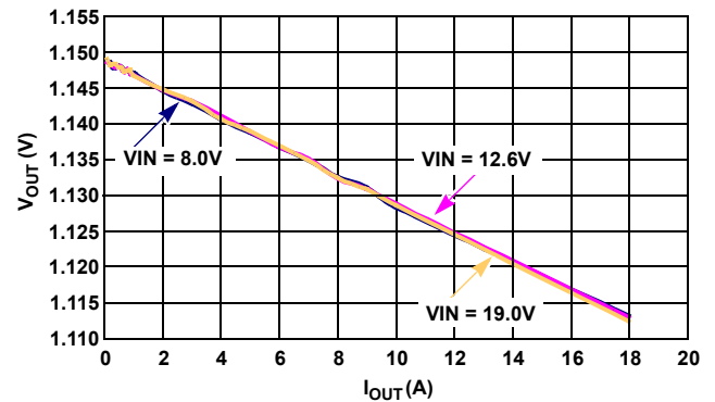
FIGURE 7. ACTIVE MODE LOAD LINE, 1 PHASE, DE, \text{PSI}_L = LOW, \text{VID} = 1.15V
