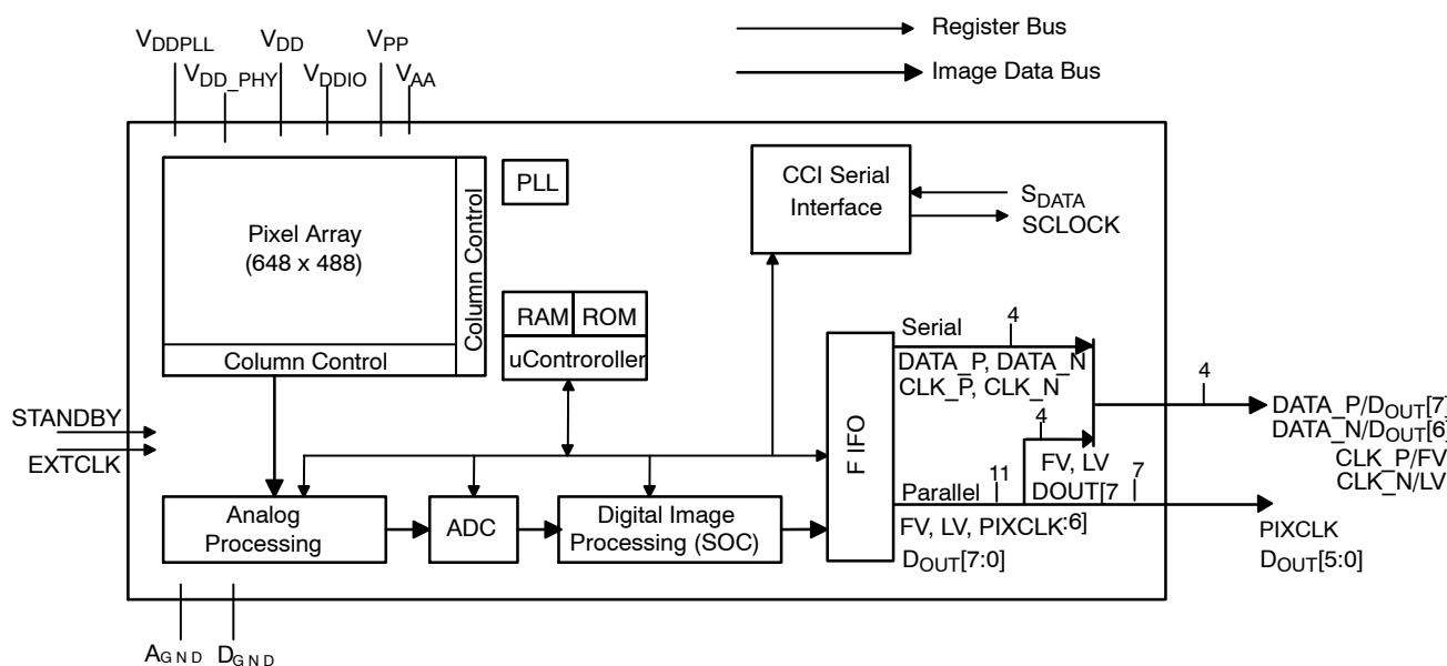
Figure 1. MT9V115 Block Diagram
