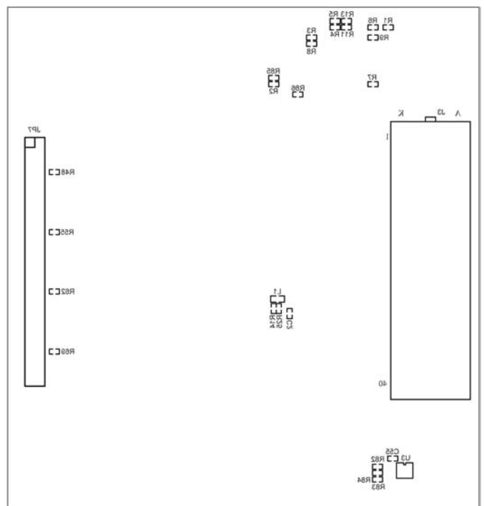
Silkscreen Bottom
