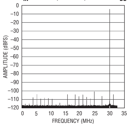
LTM9008-14: 64k Point FFT, f_{IN} = 30\text{MHz} , -1\text{dBFS} , \text{SENSE} = V_{DD}
