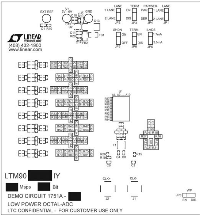
Silkscreen Top
