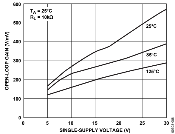
Figure 8. Open-Loop Gain vs. Single-Supply Voltage
