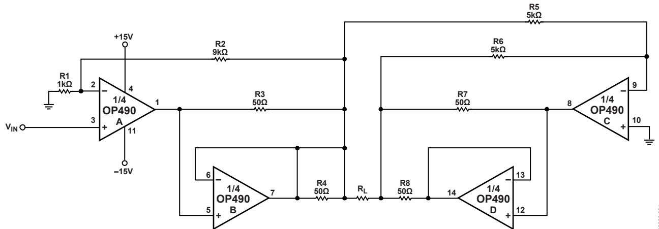
Figure 24. High Output Amplifier
