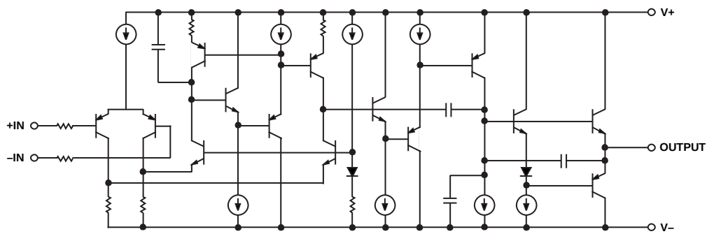
Figure 3. Simplified Schematic
