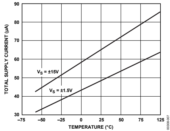
Figure 7. Total Supply Current vs. Temperature
