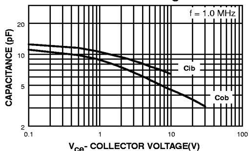
Input and Output Capacitance vs Reverse Voltage
