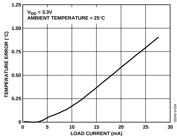
Figure 20. TMP05 Temperature Error vs. Load Current
