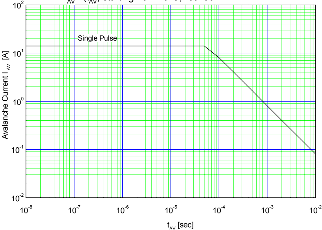
Maximum Avalanche Current Pulsewidth I_{AV}=f(t_{AV}): \text{starting Tch}=25^{\circ}C, V_{CC}=50V
