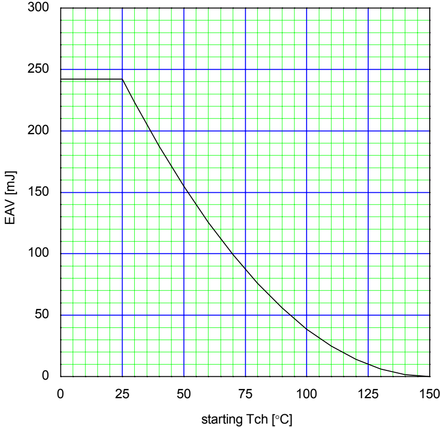
Maximum Avalanche Energy vs. starting Tch E(AV)=f(\text{starting Tch}):V_{CC}=50V, I(AV)\leq 14A
