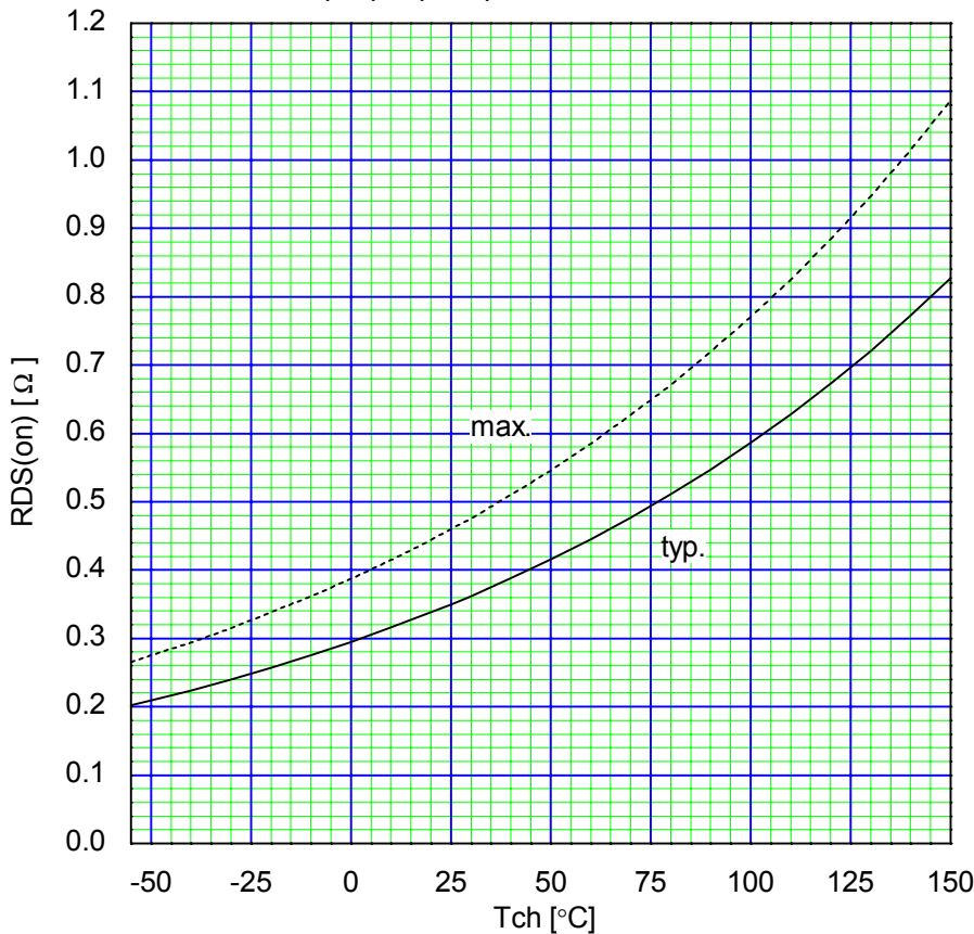
Drain-Source On-state Resistance R_{DS(on)}=f(T_{ch}):I_D=7A,V_{GS}=10V
