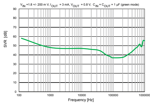
Figure 29. SVR vs. frequency (green mode)
