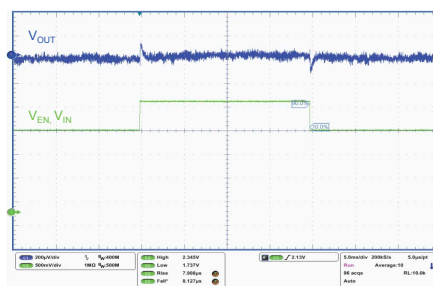
Figure 44. Load transient ( I_{OUT} = 0 to 300 mA, auto green mode)
