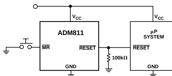
Figure 1. Typical Operating Circuit
