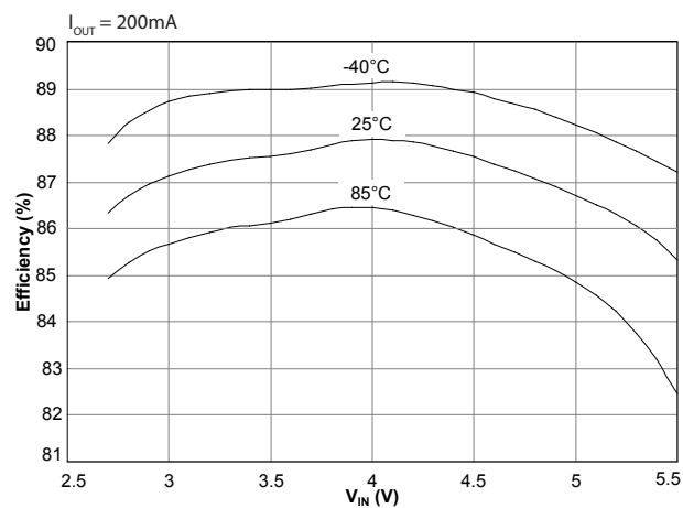
Efficiency vs. V_{IN} ( V_{OUT} = 1.8V )
