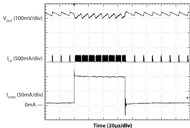
Load Transient Response — 10 to 100mA
