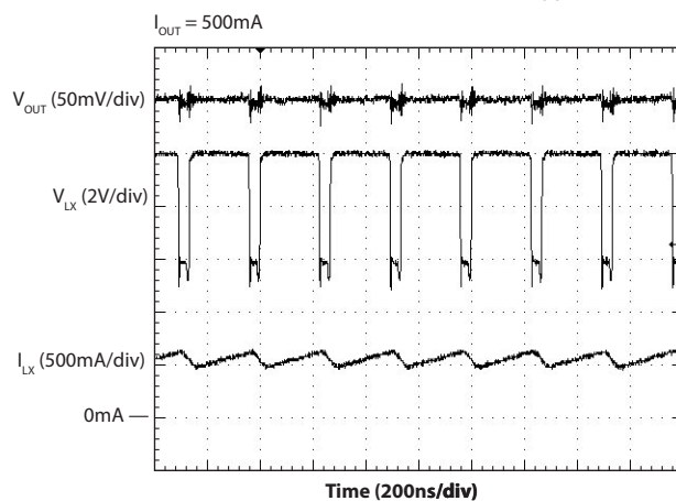
Heavy Load Switching — V_{OUT} = 3.3V
