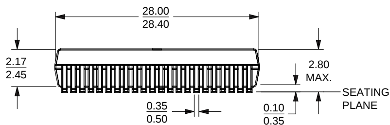
SIDE VIEW
