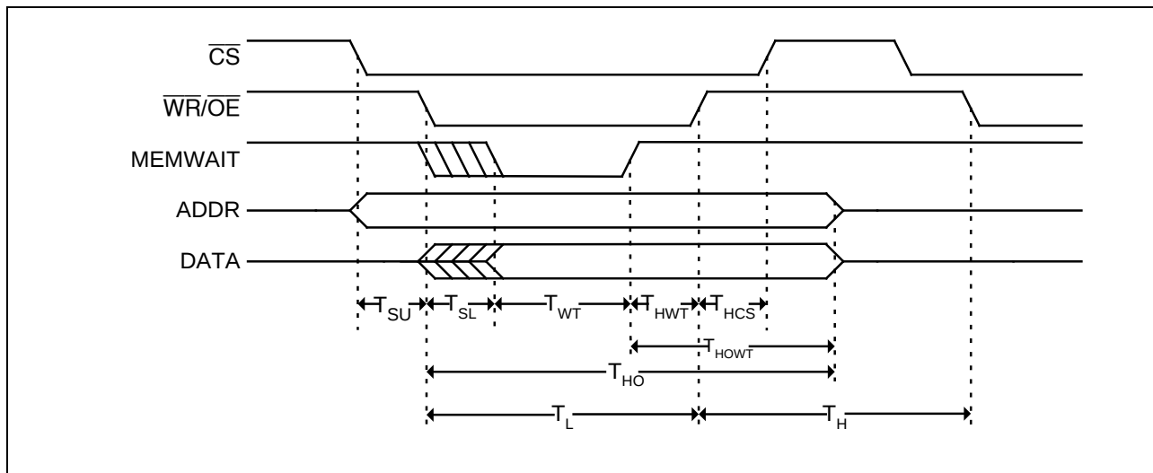
Figure 8: Host Interface Timing Diagram
