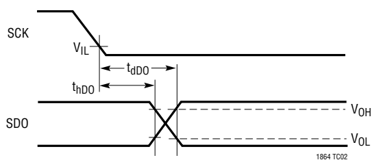
Voltage Waveforms for SDO Delay Times, t_{dpo} and t_{hpo}
