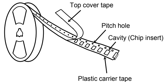
Paper Carrier Tape & Reel (Type 2)
