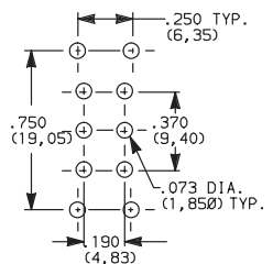
PC MOUNTING
