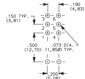
PC MOUNTING
