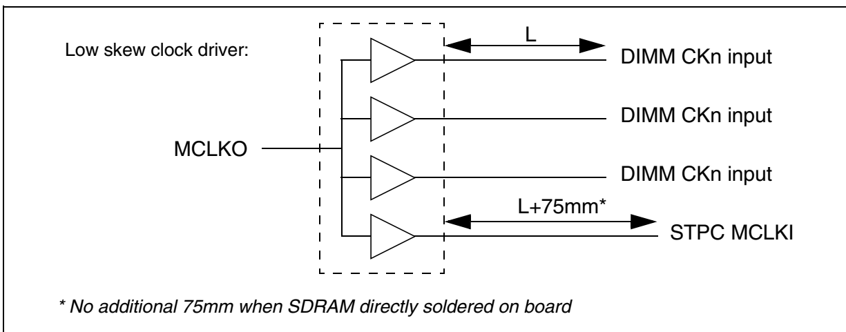
Figure 6-20. Clock Routing
