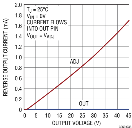
LT3060 Reverse Output Current
