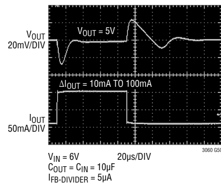
LT3060-5 Transient Response, C_{FF} = 10\text{nF}
