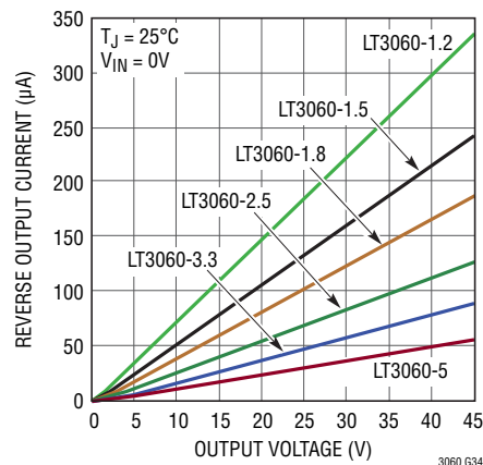
LT3060-1.2/-1.5/-1.8/-2.5/-3.3/-5 Reverse Output Current
