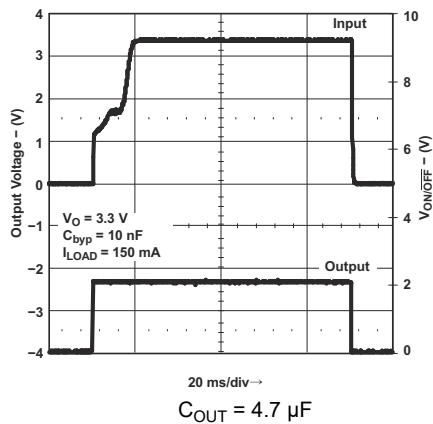
Figure 7-23. Turn-On Time
