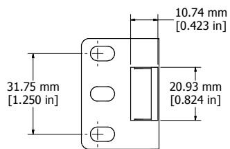
(1) REAR SUPPORT BRACKET FRONT VIEW
