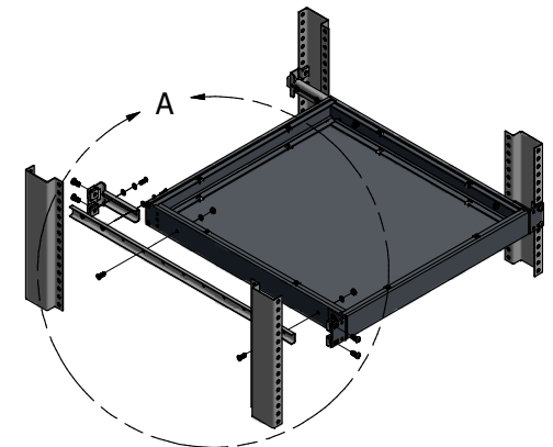
ISOMETRIC VIEW (EXPLODED)
