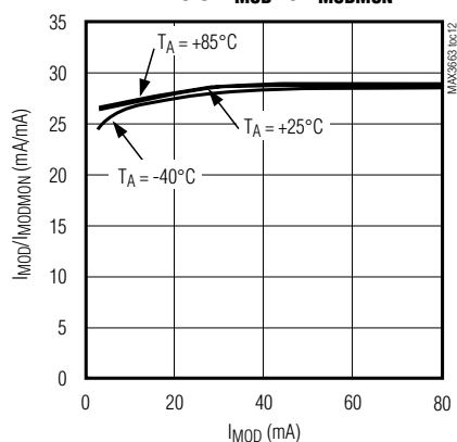
RATIO OF I_{MOD} vs. I_{MODMON}
