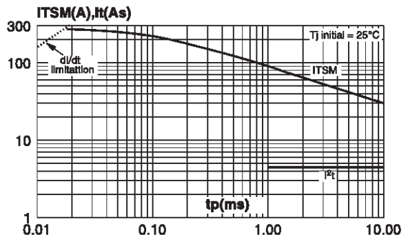
Fig. 9: Non-repetitive surge peak on-state current for a sinusoidal pulse with width t_p < 10\text{ ms} , and corresponding value of I_t .
