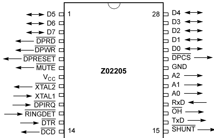
Figure 2. Z02205 Pin Diagram, SOIC/DIP
