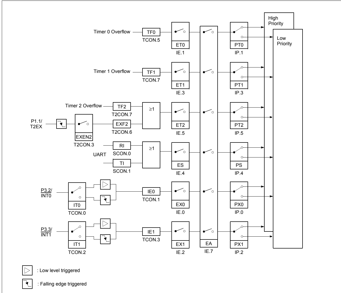
Figure 3. Interrupt Structure
