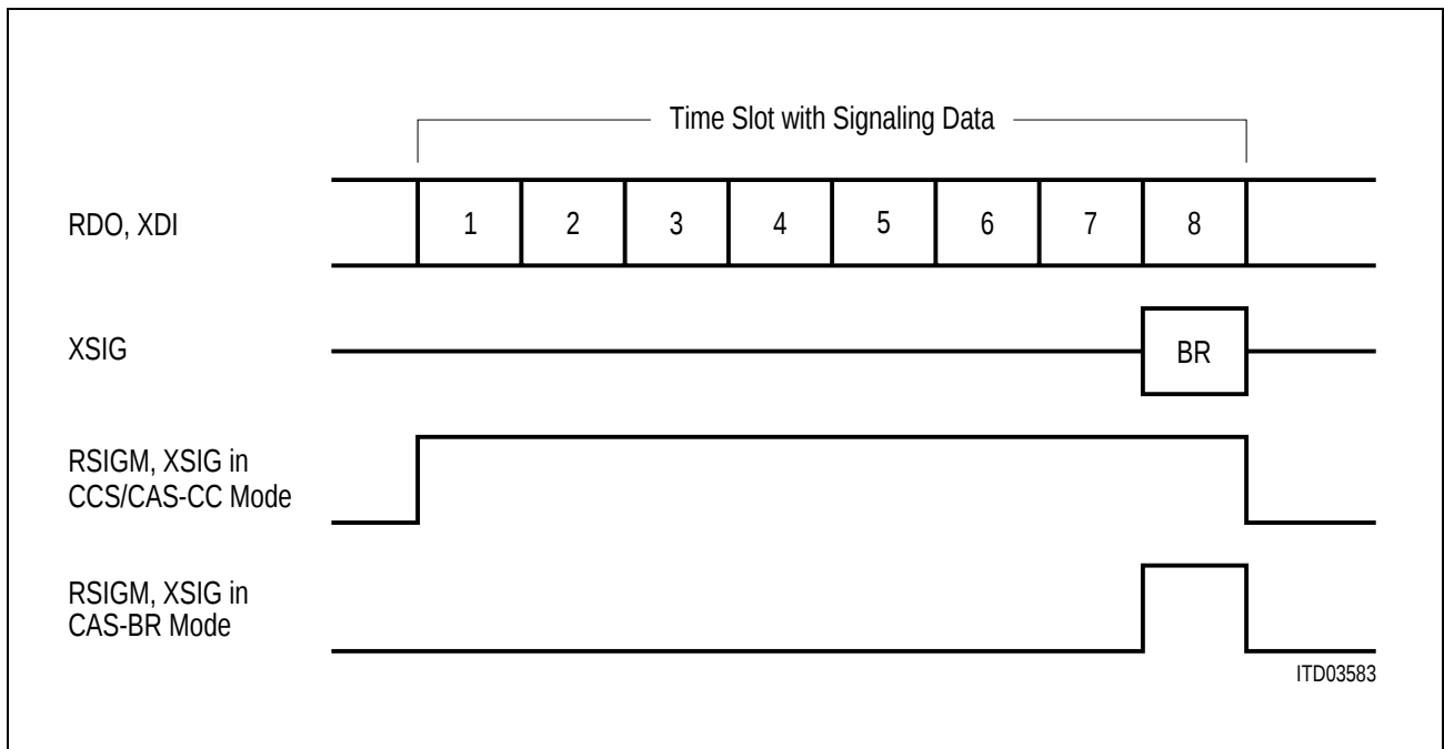
Signaling Markers in 2/4-Mbyte/s System Interface Mode
