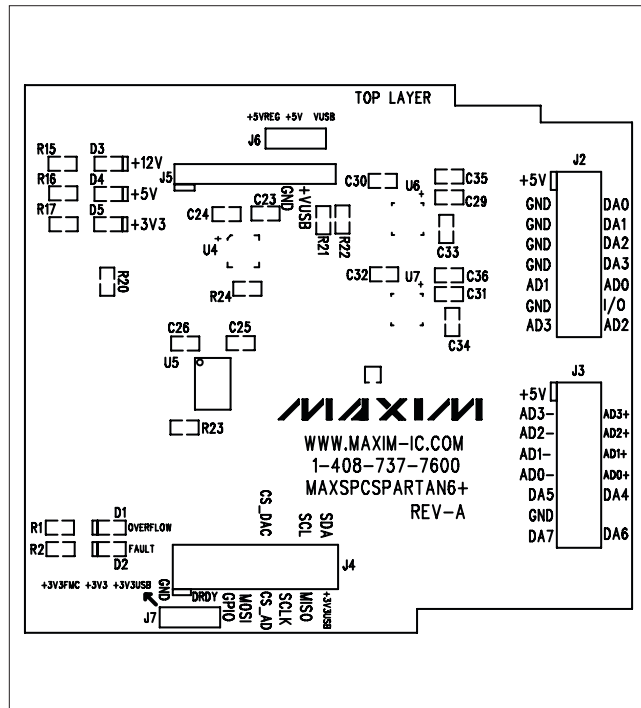
Figure 2. MAXSPCSPARTAN6+ Component Placement Guide—Component Side
