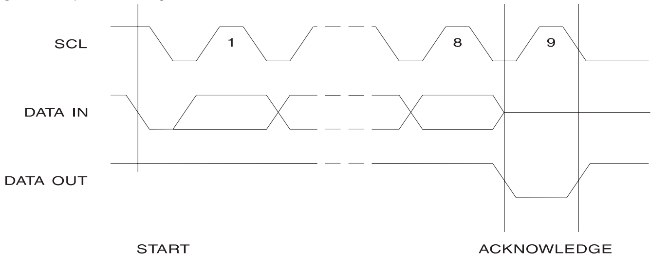
Figure 6. Output Acknowledge
