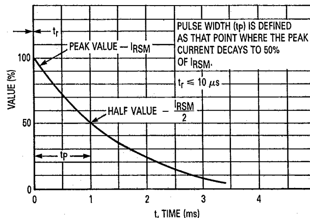
Figure 2. Pulse Waveform
