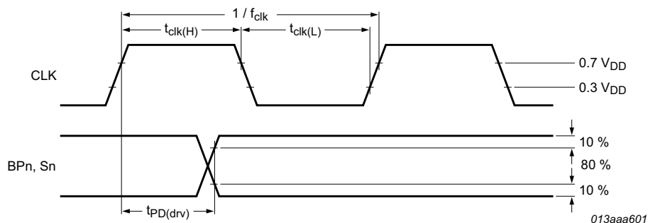
Fig 24. Driver timing waveforms
