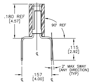
(-06) DUAL ENTRY
