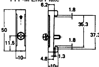
PFP-M End Plate
