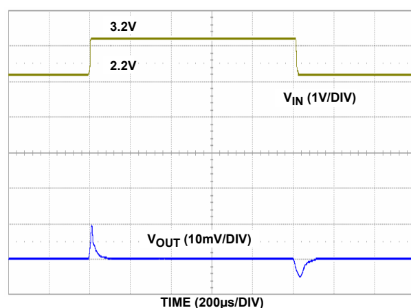
FIGURE 34. LINE TRANSIENT
