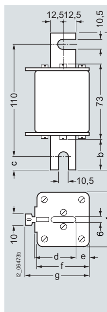
Type Dimensions (mm) a b 3NC3 2...-6 52 50 3NC3 3...-6 73 71
