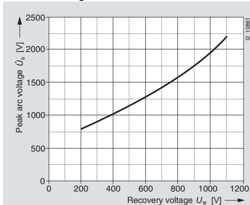
Peak arc voltage
