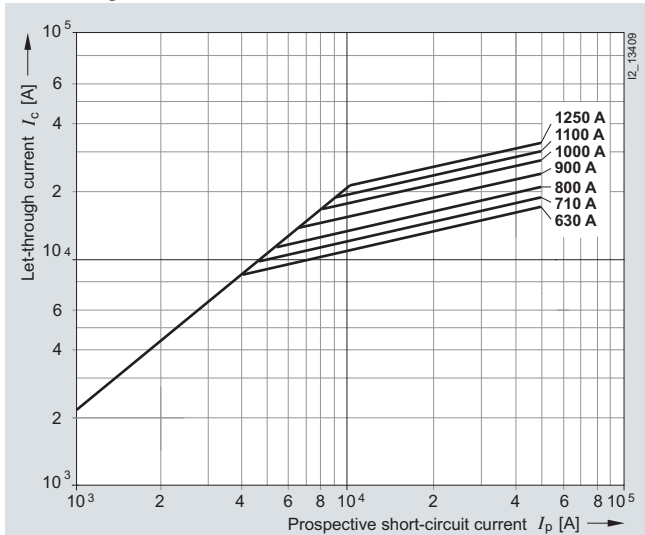
Let-through characteristic curves
