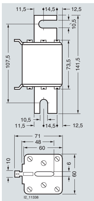
Type Dimensions (mm) a b c d 3NC3 2...1 102 51 78 40 3NC3 3...1 139 72 108 61
