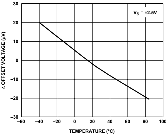
Figure 41. \Delta Offset Voltage vs. Temperature
