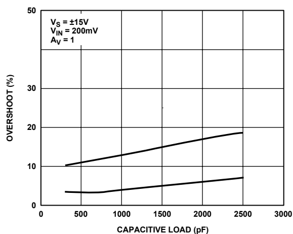
Figure 10. Overshoot vs. Load Capacitance
