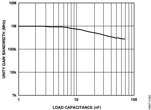
Figure 52. Unity Gain Bandwidth vs. Load Capacitance
