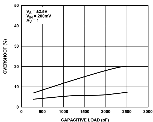
Figure 33. Overshoot vs. Load Capacitance
