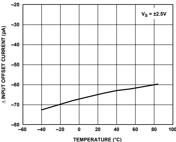
Figure 43. \Delta Input Bias Current vs. Temperature
