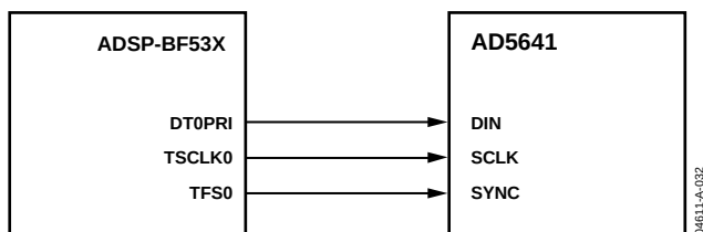
Figure 31. AD5641 to Blackfin ADSP-BF53X Interface
