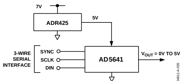
Figure 34. ADR425 as Power Supply to AD5641
