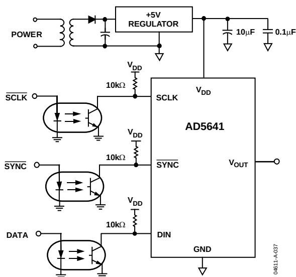
Figure 36. AD5641 with an Opto-Isolated Interface
