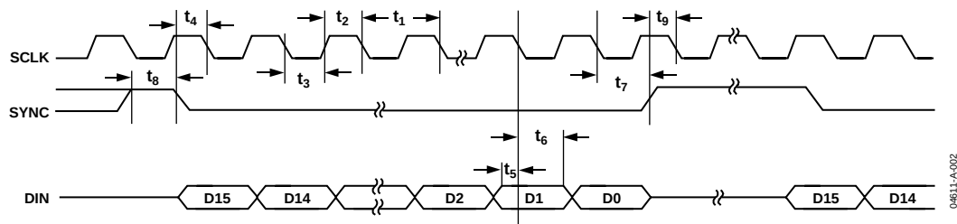
Figure 2. Timing Diagram
