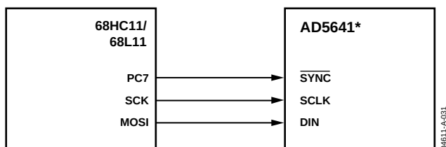
Figure 30. AD5641 to 68HC11/68L11 Interface
