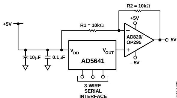
Figure 35. Bipolar Operation with the AD5641
