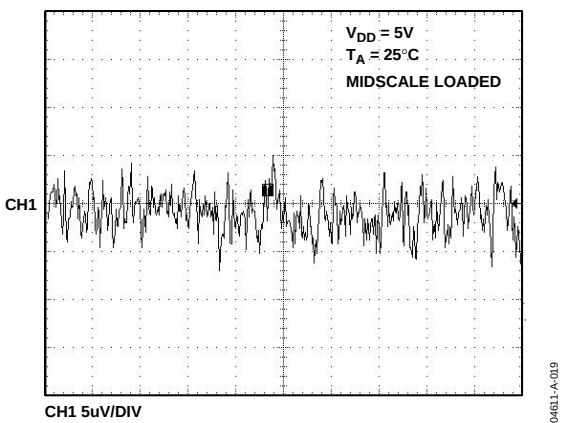
Figure 19. 1/f Noise, 0.1 Hz to 10 Hz Bandwidth
