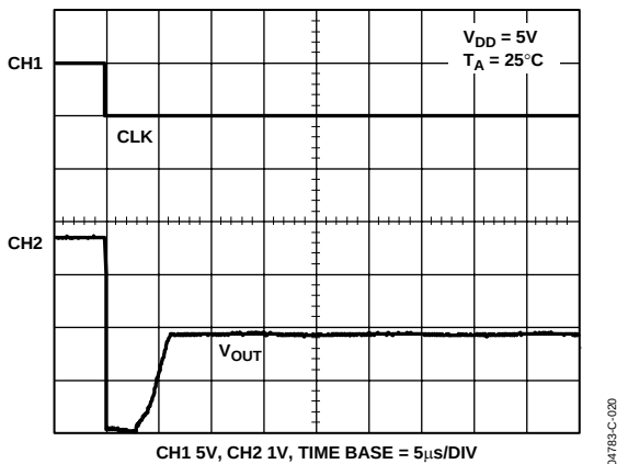
Figure 20. Exiting Power-Down
