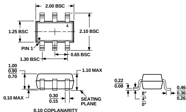
Figure 37. 6-Lead Plastic Surface Mount Package [SC70] (KS-6)
