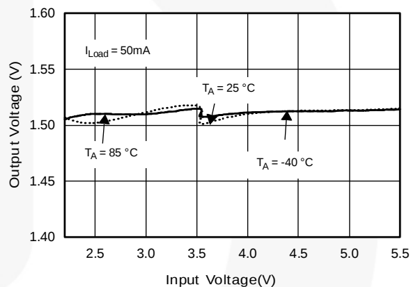
Figure 7. Line Regulation
