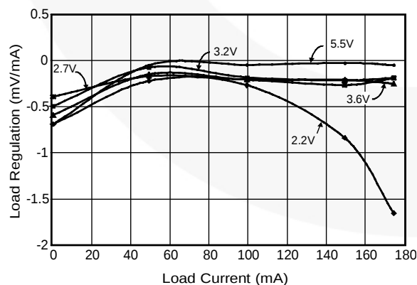
Figure 8. Load Regulation
