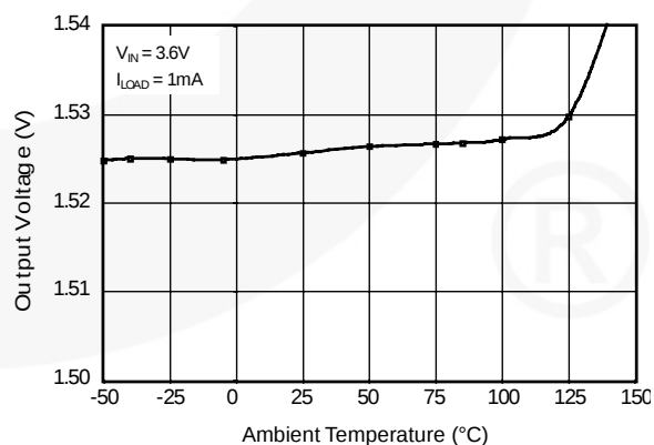
Figure 9. Thermal Regulation
