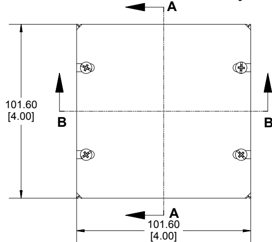
Bottom View of Assembly
